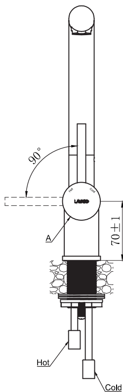
Front
